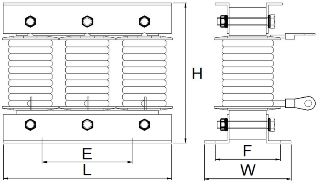
20A-150A Drawing
